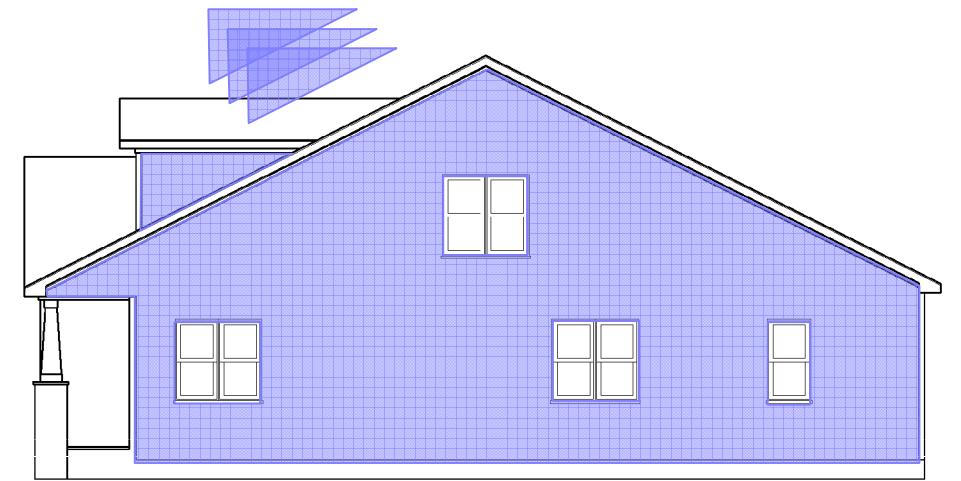
RIGHT ELEVATION 1/8" = 1'-0"
